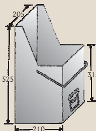
Fuel Carrier Part No. 01429
