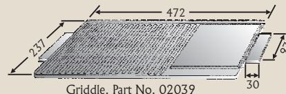
Griddle. Part No. 02039
