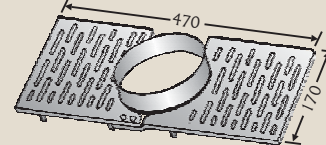
Trivet. Part No. 02040
